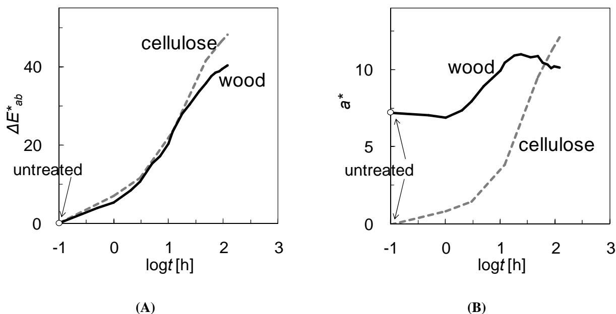
Fig. 3 Changes of (A) \Delta E^*_{ab} and (B) a^* value in wood and cellulose that occur during heat treatment at 180 °C.
